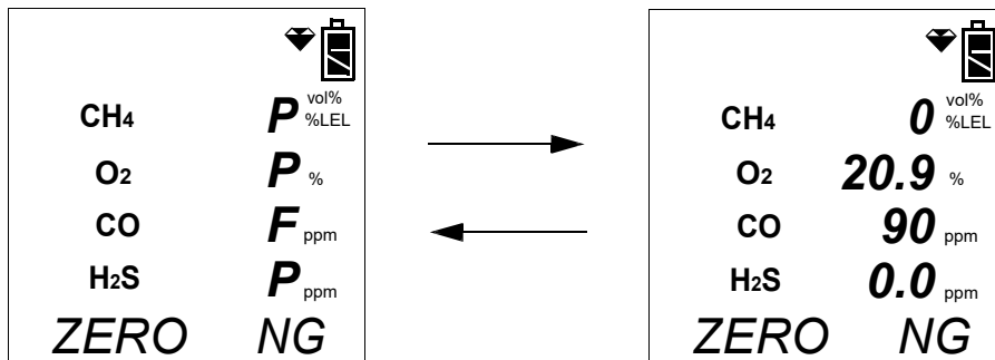
Figure 28: Failed Fresh Air Adjustment, %Volume Sensor Installed and GAS Menu Item in Edit Mode Set to ALL
