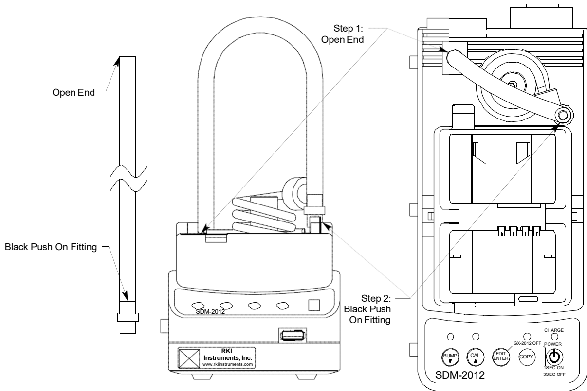
Figure 13: Installing the Exhaust Line
