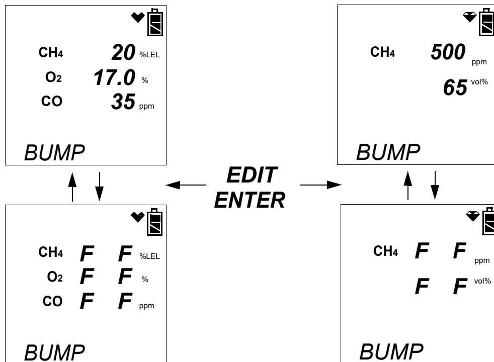
Figure 41: Failed Bump Test and Calibration, %Volume Sensor Installed and GAS Menu Item in Edit Mode Set to ALL
