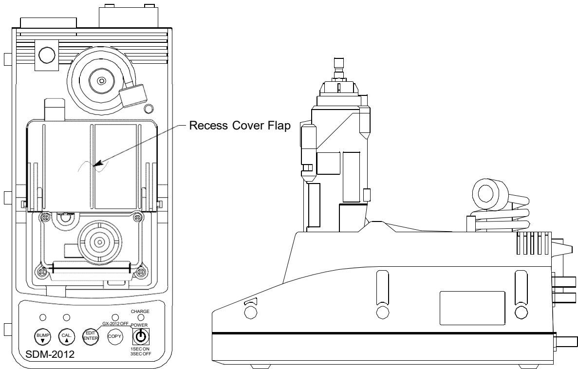
Figure 9: Instrument Panel with Lithium Ion Instrument Installed
