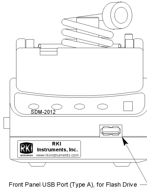
Figure 12: Front Panel
