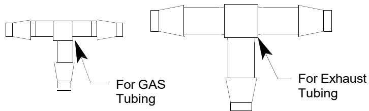
Figure 6: T-Fittings
