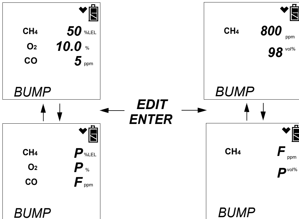
Figure 37: Failed Bump Test, AUTO CAL OFF, %Volume Sensor Installed and GAS Menu Item in Edit Mode Set to ALL
