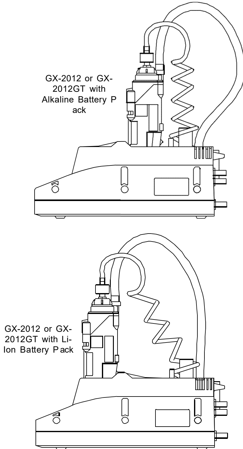
Figure 15: Inserting the GX-2012
