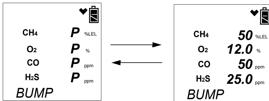
Figure 18: Screen Indication for Passed Bump Test, Standard 4-Gas GX-2012 or GAS Menu Item in Edit Mode Set to Std
