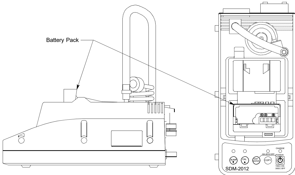
Figure 47: Inserting the Battery Pack for Charging
