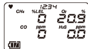
Measurement screen
