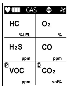
Detection target gas names
