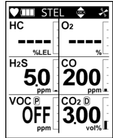
STEL alarm setpoint display
