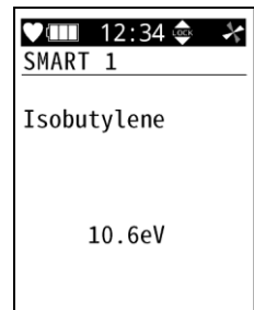
VOC gas name / Sensor type display (Displayed only if a VOC sensor is installed)
