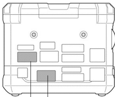
Type examination certificate mark location
