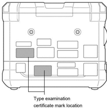
Typical nameplates for explosion-proof electrical equipment type certified (Japan EX) models
