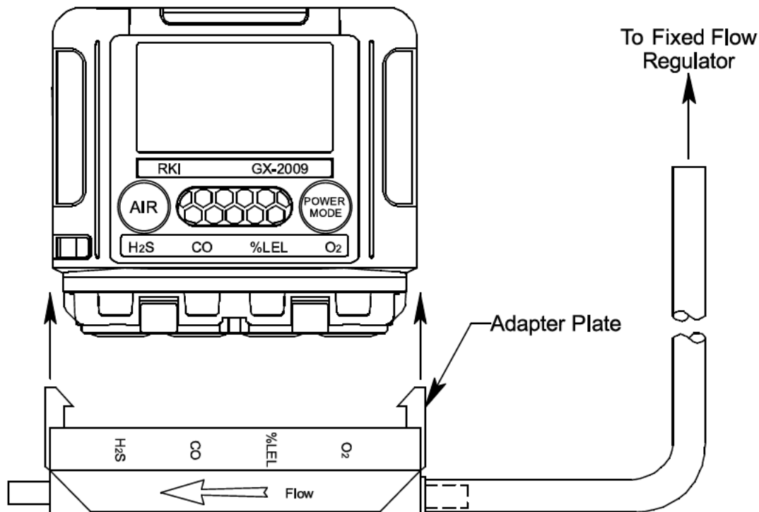
Figure 12 : Installing the Adapter Plate, One Cal
