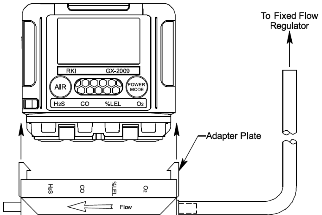
Figure 10 : Installing the Adapter Plate, Auto Cal
