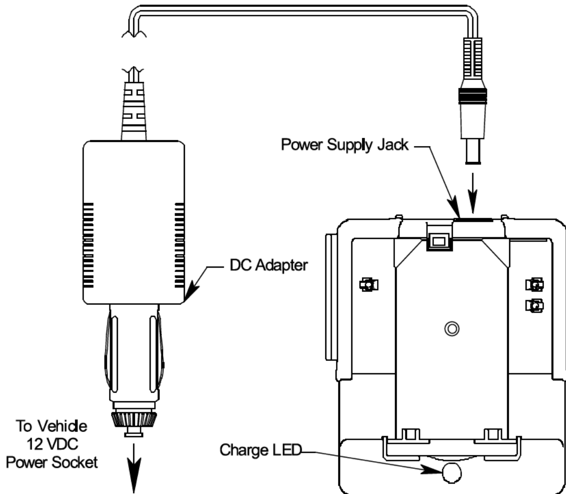
Figure 14 : Connecting the Charging Station's DC Adapter
