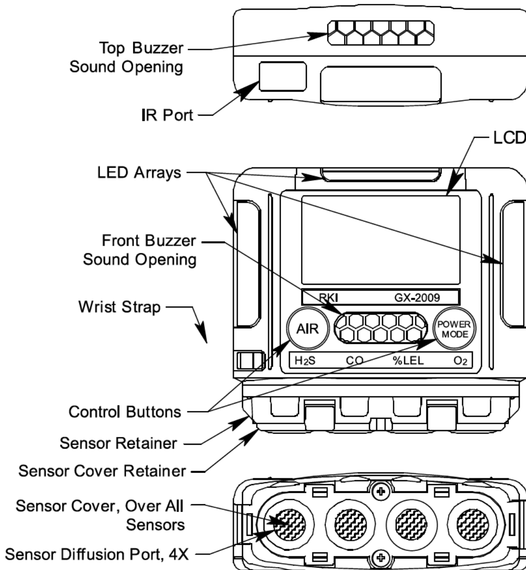
Figure 1 : GX-2009, Front & Bottom View
