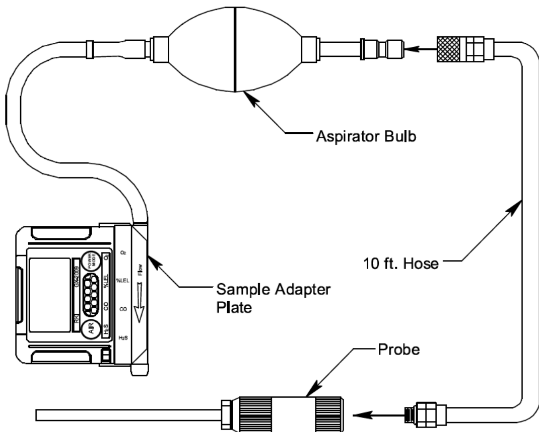
Figure 8 : GX-2009 Aspirator Adapter
