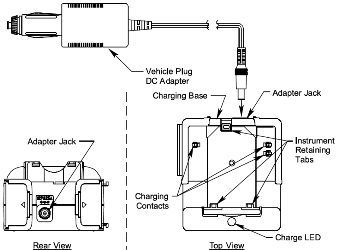
Figure 7 : GX-2009 DC Powerd Charging Station
