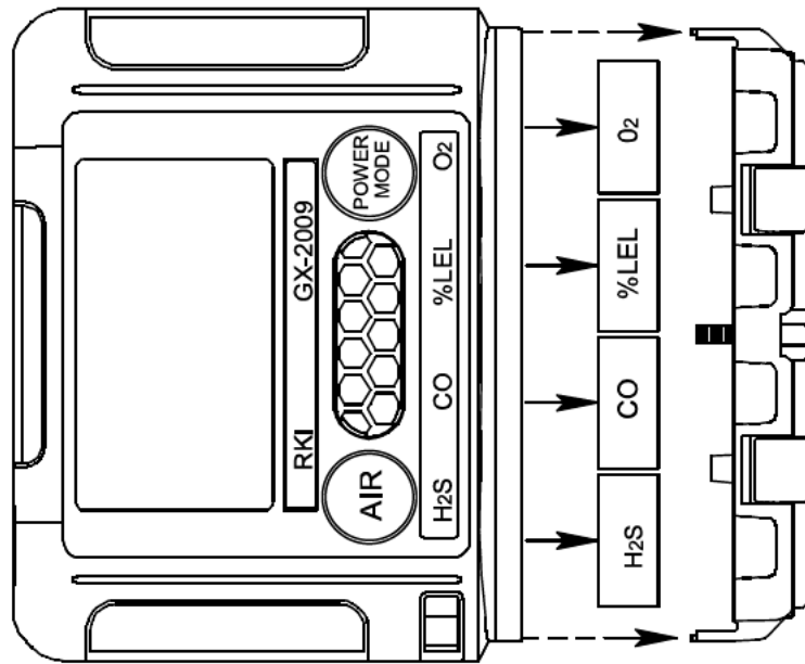
Figure 22 : Removing the Sensor Retainer to Replacing Sensor
