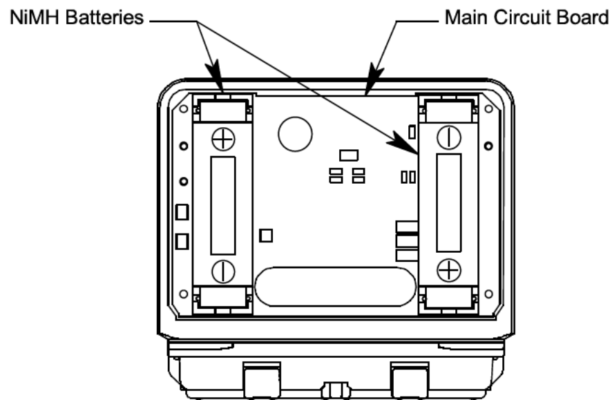
Figure 19 : NiMH Batteries
