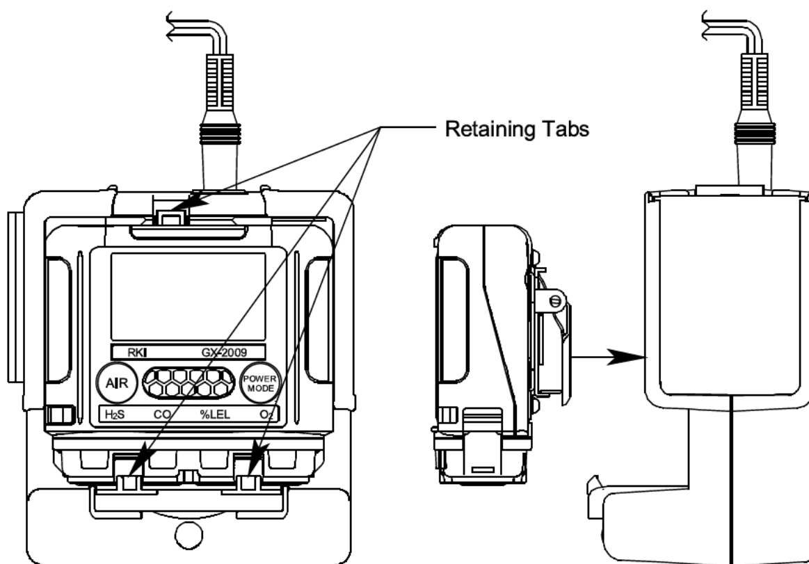
Figure 15 : Putting the GX-2009 in the Charging Base
