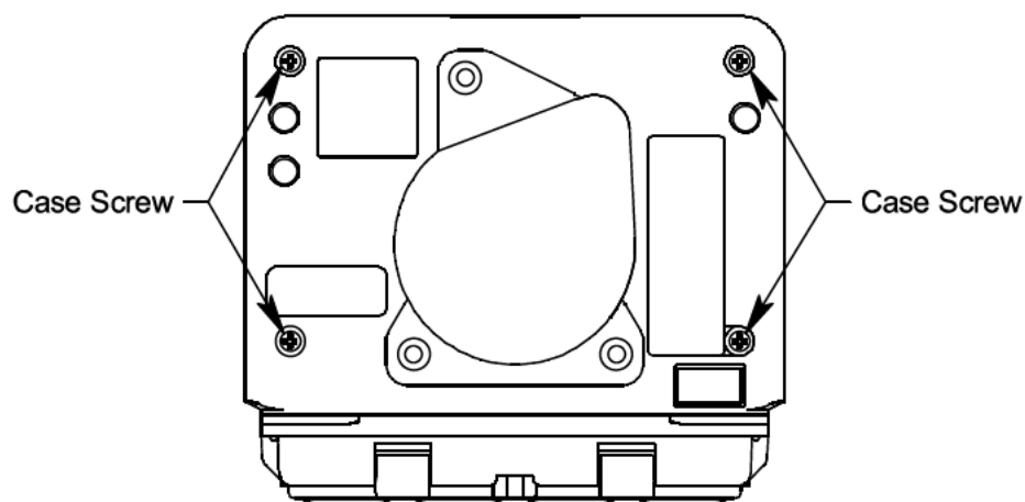
Figure 16 : Removing the Case Screws
