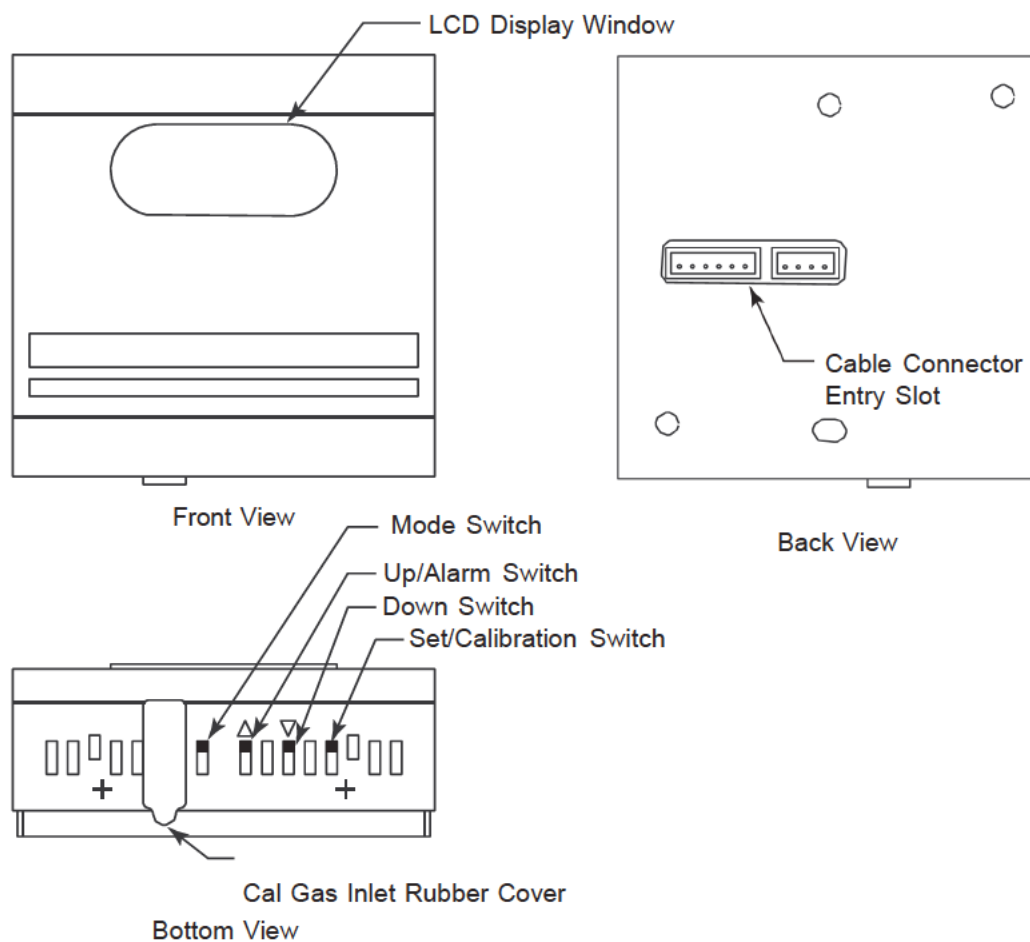
Figure 1: Component Location of the RI-215A
