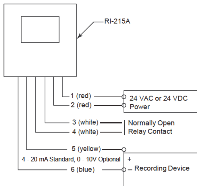
Figure 3: General Wiring Diagram of the RI-215A
