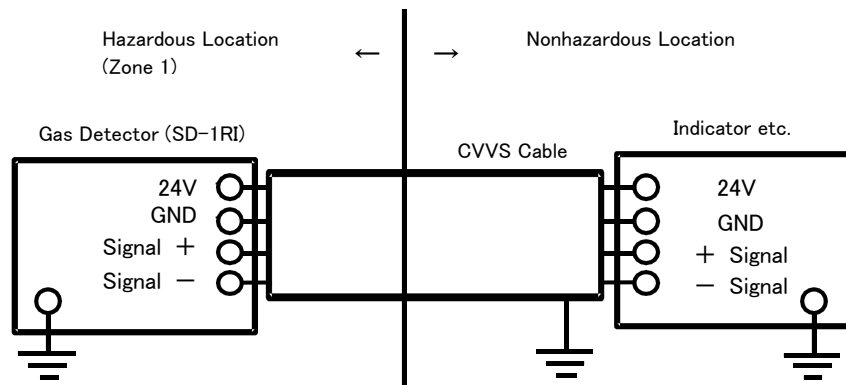
Installation Diagram
