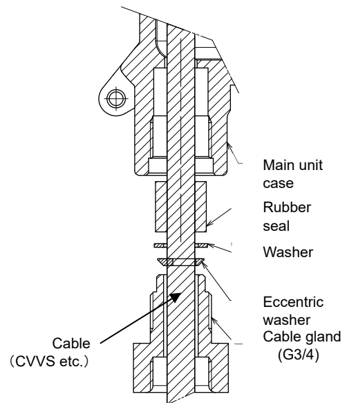
Cable gland section view
