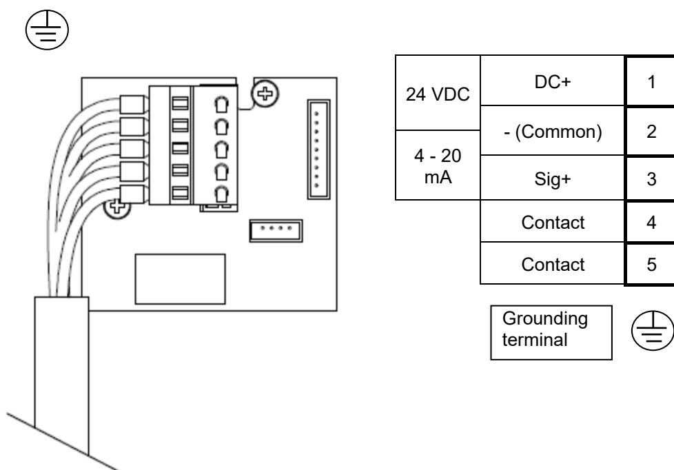
<Figure of Terminal Plate>
