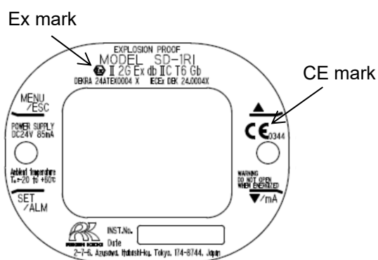
ATEX/IECEX, CE marking type name plate
