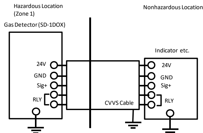
Installation Diagram
