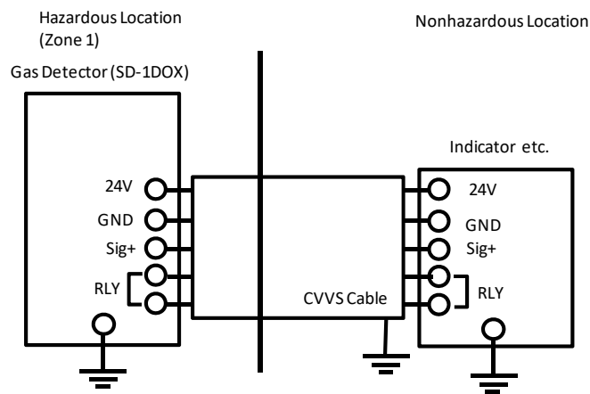
Installation Diagram
