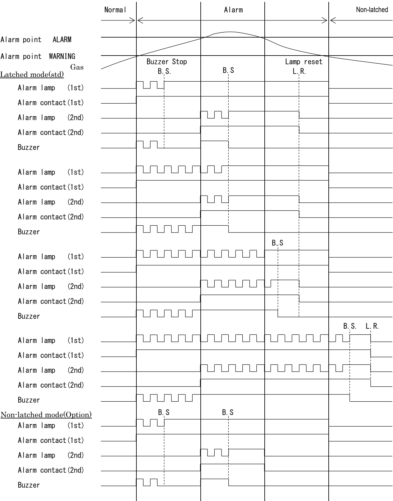
Timing chart
