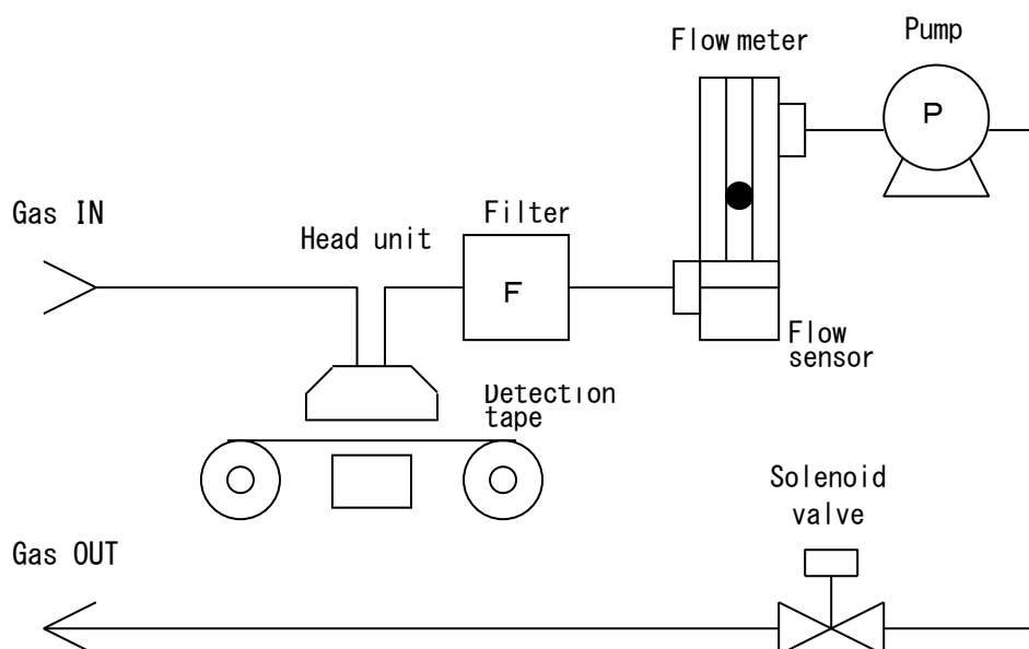
Piping diagram
