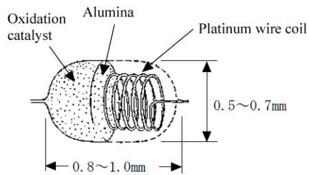
Structure diagram
