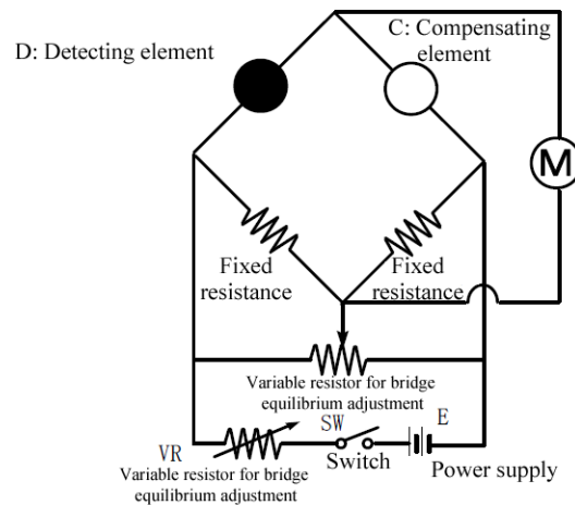
Basic circuit
