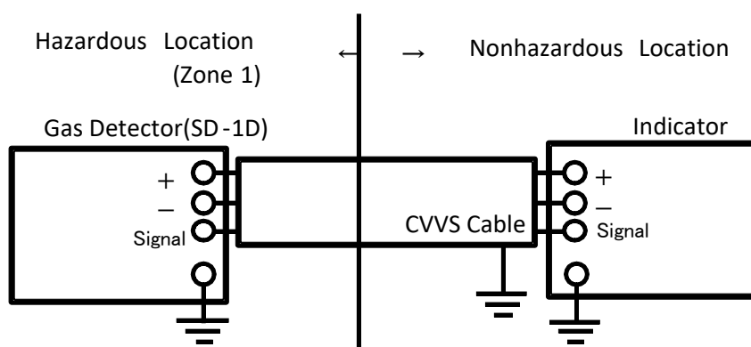
Installation Diagram
