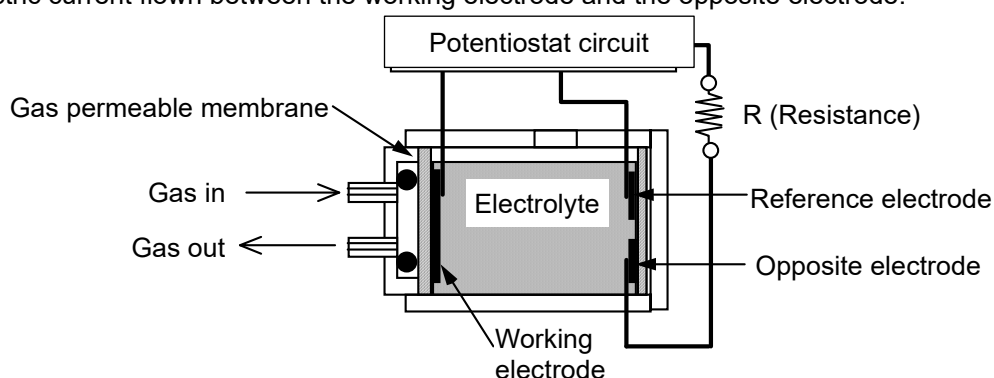
Structure diagram
