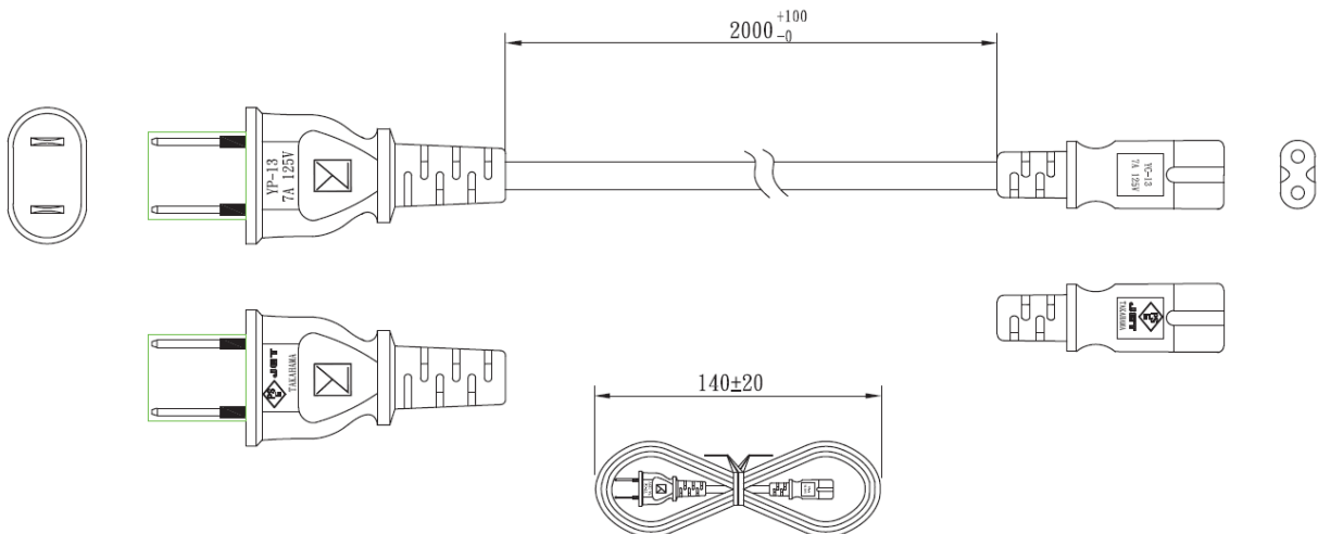
FRONT-VIEW
