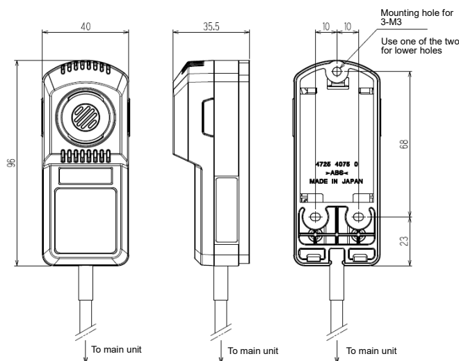
Remote sensor
