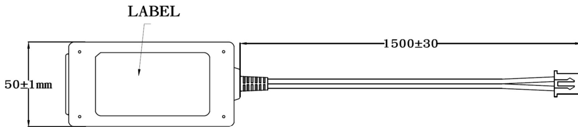
BOTTOM VIEW
