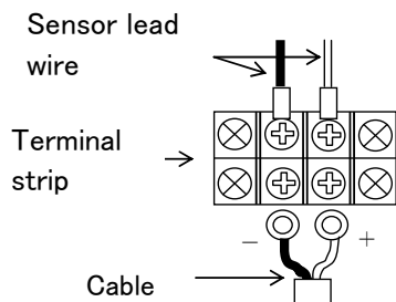
Cable connection
